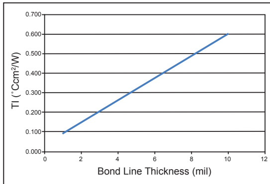
PTM6000 Thermal Impedance vs. Bond Line Thickness
